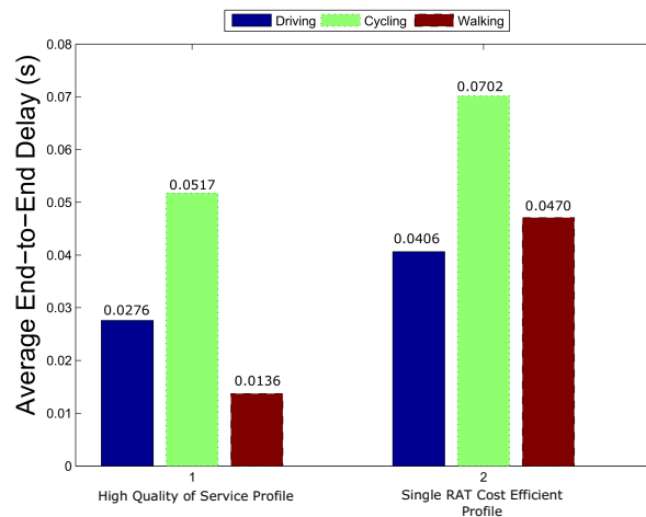
Figure 8: Comparison of End-to-End Delay for WiFi only profile vs High QoS profile
