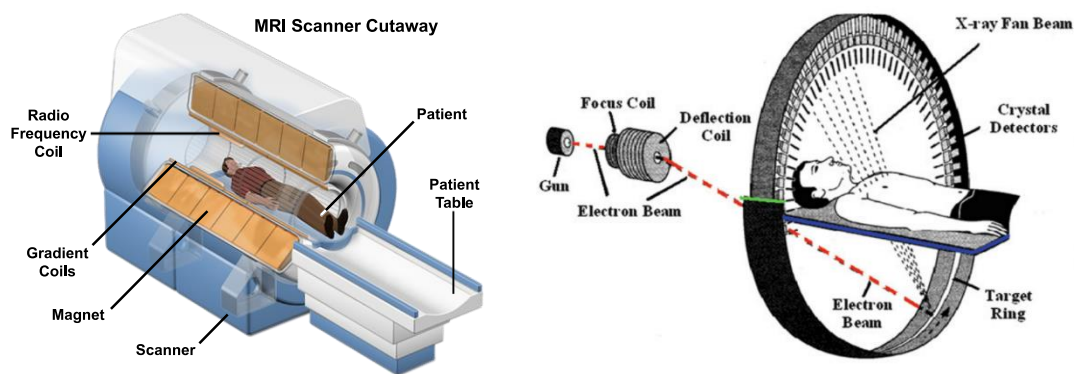
Figure 1-7 – MRI (left) versus CT-scan (right) . MRI captures the photons released by hydrogen atoms of the body after a radio waves impulse while CT-scan relies on X-ray. 3D Images from both modalities will be analysed in this thesis. Illustrations taken from [35] and [36].
