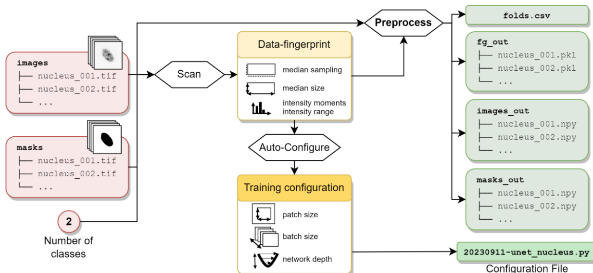
Figure 3-13 – Auto-configuration and Preprocessing of training dataset for 3D segmentation. Image and mask folders ( red, left ) are scanned to extract their data-fingerprint. The data-fingerprint is used to preprocess the images and masks and to automatically configure the future training ( yellow, centre ). The outputs of these two steps ( green, right ) are: a CSV file ( folds.csv ) describing which files will be used for training or validation, a Configuration File, the pre-processed images ( images_out ) and masks ( masks_out ), and the location of the foreground voxels ( fg_out ).
