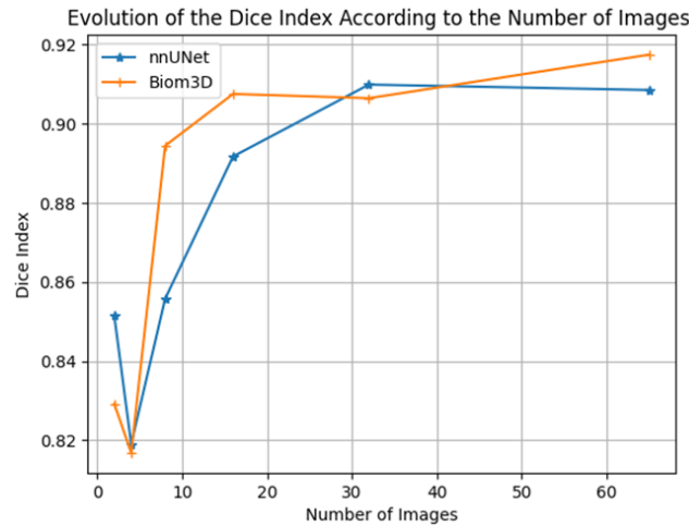
Figure 4-2 – Preliminary comparison between Biom3d (orange) and nnU-Net (blue). The Dice scores are obtained using the same testing set while training on set training sets of increasing sizes (2, 4, 8, 16, 32 and 65 images). The curves drop down between 2 and 4 images probably due to bad annotations.
