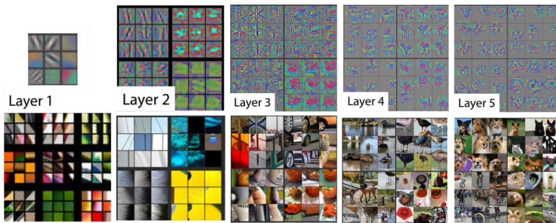
Figure 2-5 – What does the deep learning model “sees”? Visualization of the output of some activation layers at different depth in the deep learning model ( top row ). These views have been reconstructed with a deconvolution model (inverted convolution) using the samples displayed in the bottom line. It can be noted that the deeper the layer is in the model, the more complex the patterns of attention are, shallow layers focusing on simple edges and deep layers focusing on complete objects. Illustration adapted from [65].
