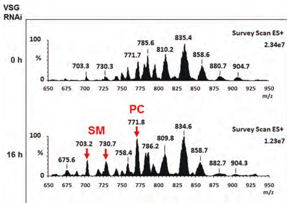
FIGURE 9 Lipidomic analysis of Trypanosoma brucei in the presence or absence of VSG RNAi for 16 hours. Survey ESI-MS in positive ion mode (600–1000 m/z ) of lipid extracts from T. brucei VG1.1 that had been cultured in the presence or absence of VSG RNAi for 0 or 16 hours (h). The red arrows indicate the species which increase significantly upon induction of VSG RNAi, which were confirmed as being choline-phosphate containing SM or PC species (Figure S3C and Table S1)
