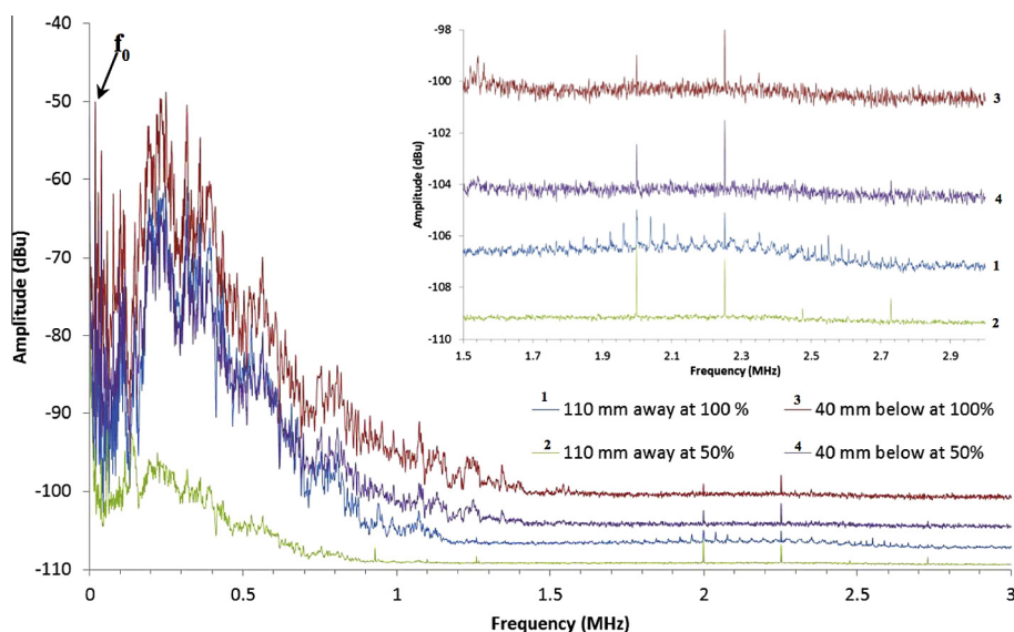
Fig. 8. Acoustic spectra in glycerine at different positions of the cavitometer (see Fig. 1) and different power settings of the transducer. Driving frequency ( f_0 ) is 20 kHz.
