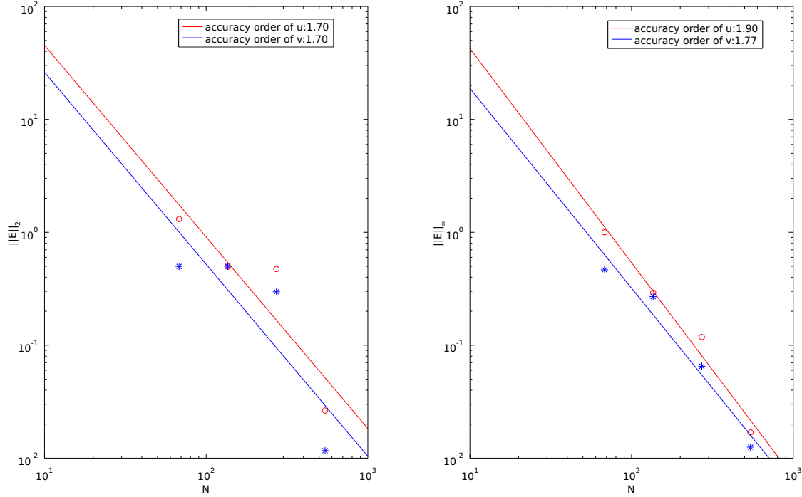
Figure 16: Example 4.3. Bestfit of the L^2 (left) and L^\infty (right) errors of u and v . The errors are obtained as the difference from a FE third order accurate solution.
