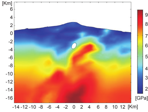
Figure 14: Example 4.3. Real profile of Etna volcano. The color scale refers to the Young modulus E .
