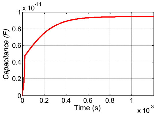
Fig. 2c) variation of C versus time
