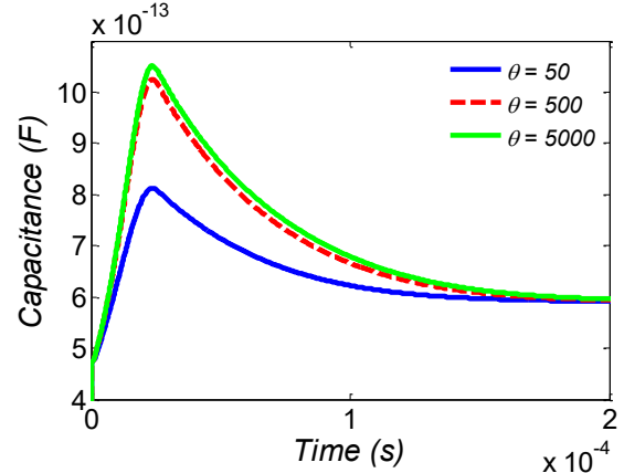
Fig. 6b) variation of C versus time for different values of \theta and x_d = 0.2
