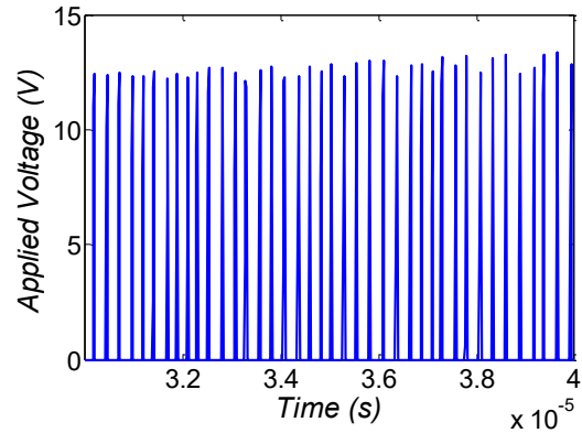
Fig. 6d) detailed view of fig 6c
