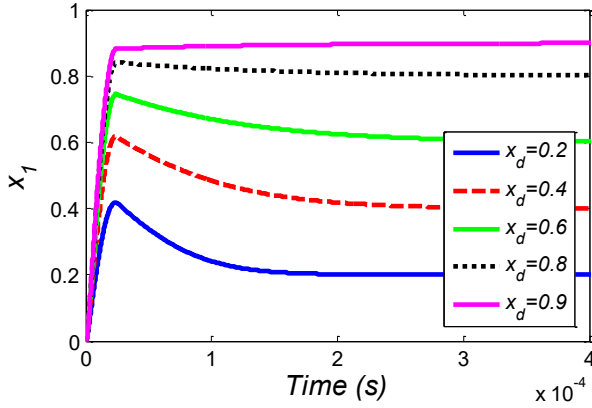
Fig. 3a) variation of x_1 versus time for different values of x_d
