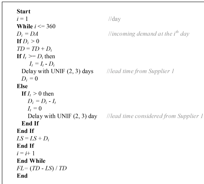
Fig. 3. Algorithm 1 - Meeting demand procedure by Supplier 1.
