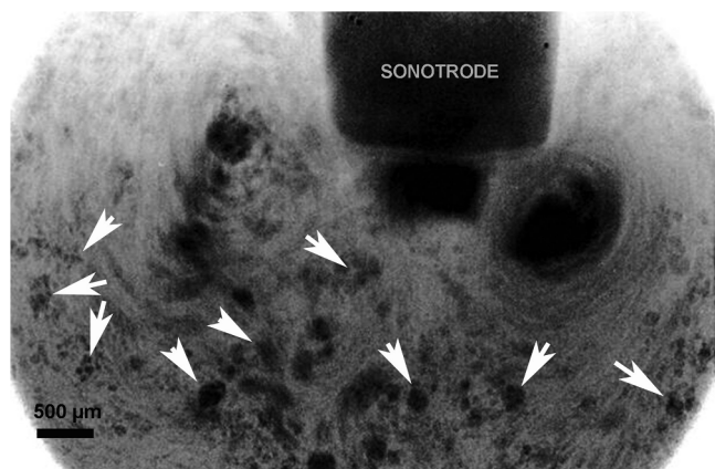
Fig. 6. Acoustic streaming and dendrite fragments (arrows) observed in a synchrotron using a Sn-30 wt% Cu alloy and 100 W acoustic power.
