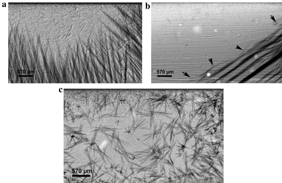
Fig. 14. Fragmentation of \text{Al}_2\text{Cu} dendrites in and Al-35 wt% Cu alloy ( in situ synchrotron X-ray study): (a) elongated dendrites growing without USP; (b) fragmentation (shown by arrows) of dendrites by acoustic streaming (ultrasonic source is above the left top corner); and (c) refined equiaxed crystals formed after the end of USP.
