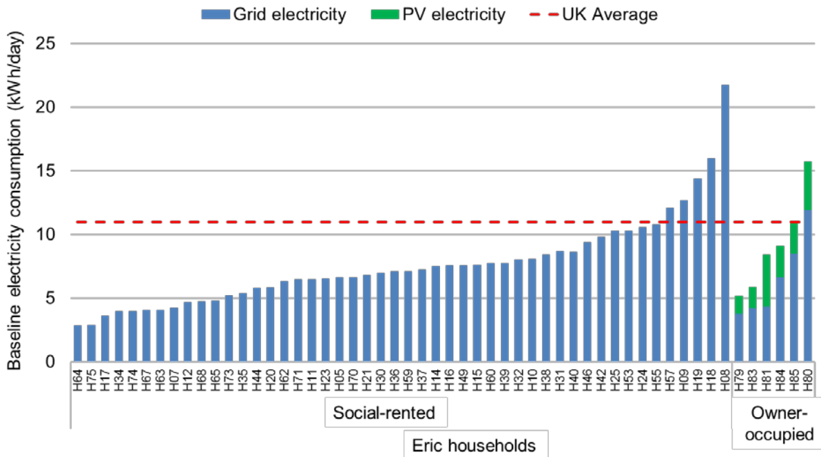
Figure 2 Baseline average daily electricity consumption for 54 dwellings: by low social housing and owner-occupied dwellings
