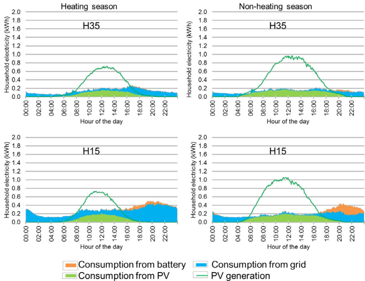
Figure 10 Household electricity consumption and generation profiles: electricity from the grid, instant consumption of PV generated electricity and PV electricity discharged from the battery in the heating season (left) and non-heating season (right) in two low consuming households
