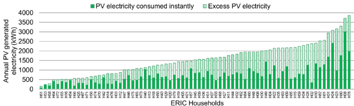
Figure 5 Annual PV generated electricity consumed instantly and excess PV electricity (n:74)
