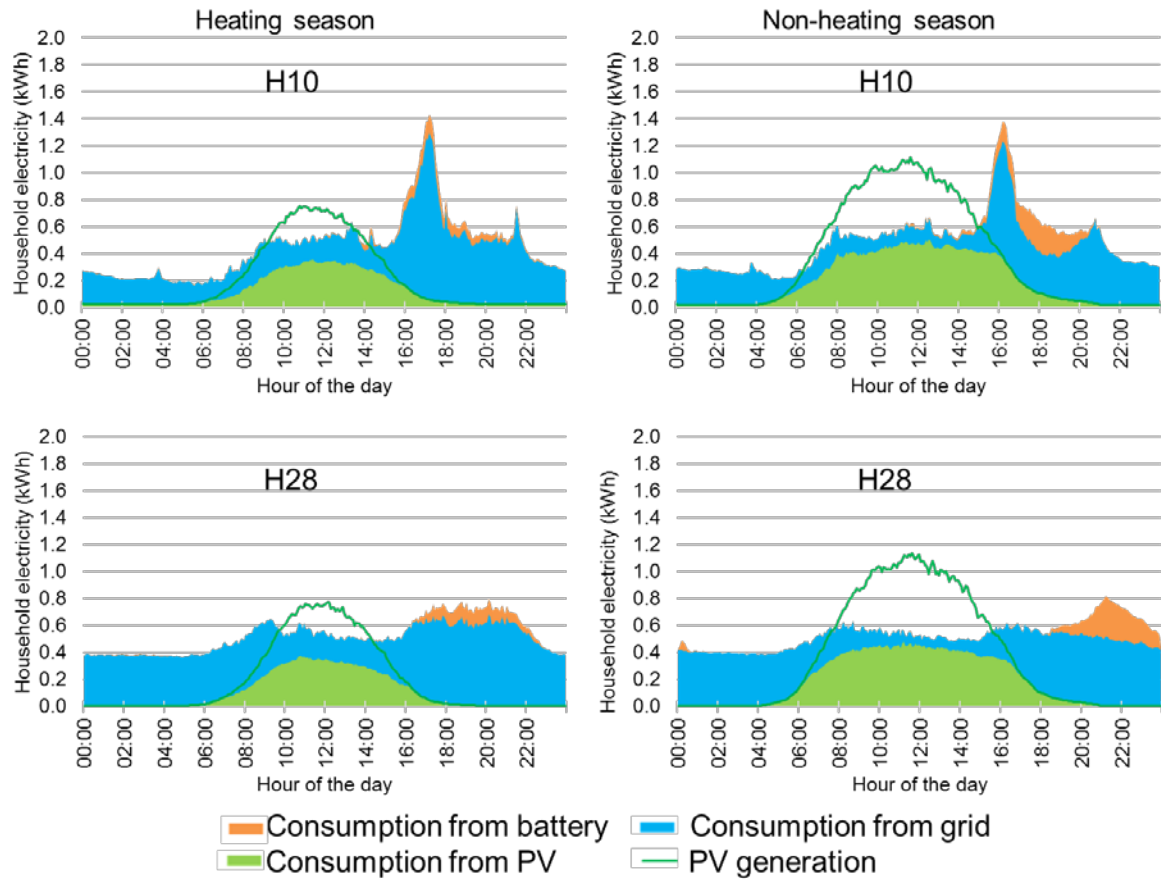
Figure 11 Household electricity consumption and generation profiles: electricity from the grid, instant consumption of PV generated electricity and PV electricity discharged from the battery in the heating season (left) and non-heating season (right) in two medium consuming households
