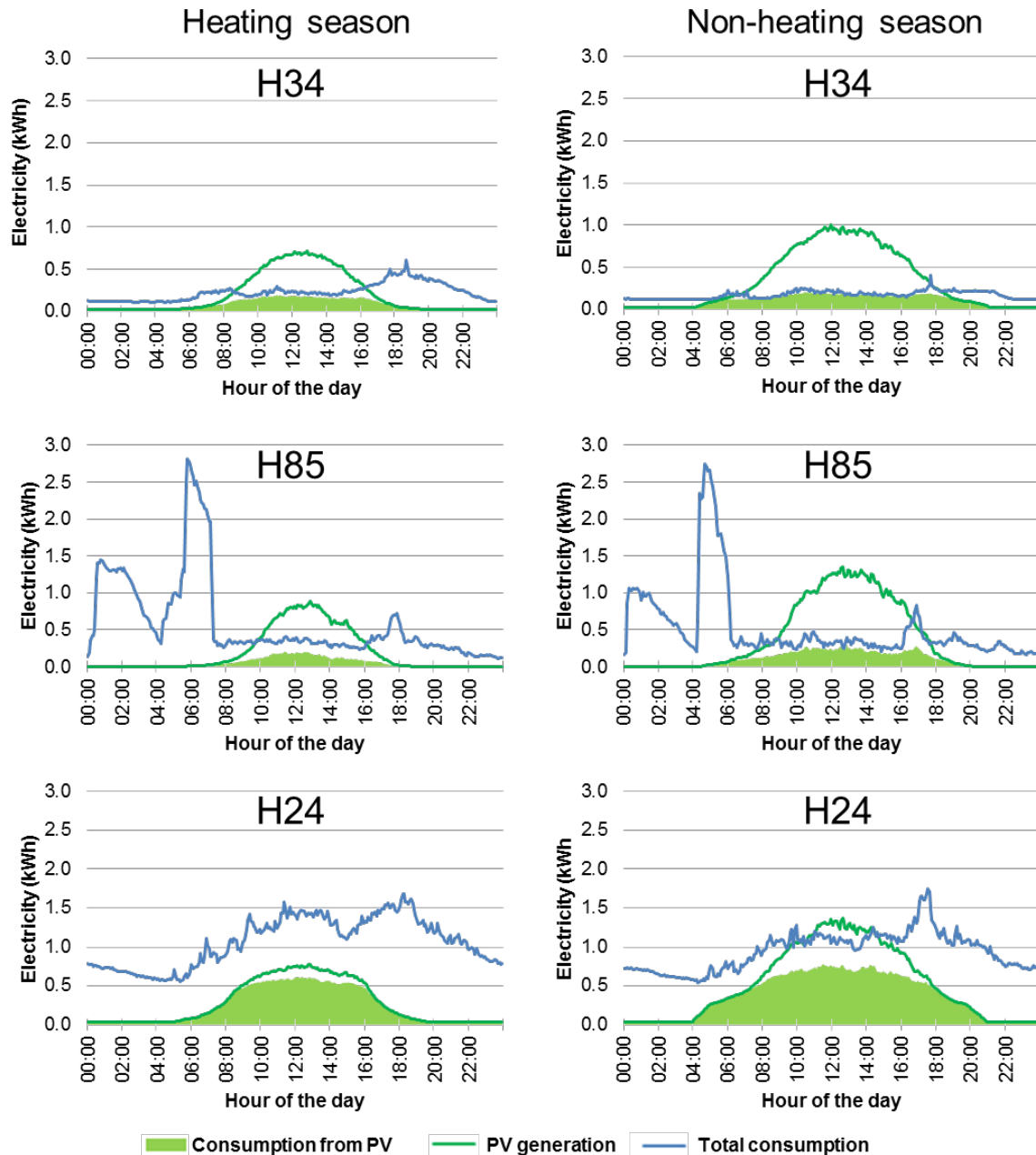
Figure 6 Instant consumption of PV generated electricity in case study households during the heating season (left) and non-heating season (right)
