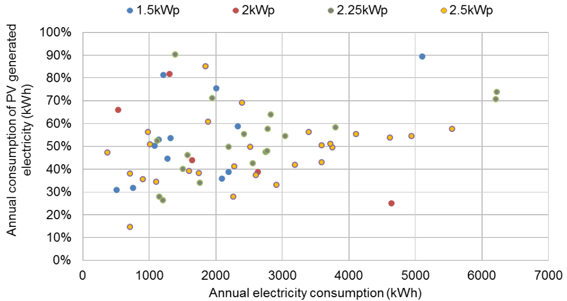
Figure 7 Scatter plot of annual dwelling electricity consumption and annual self-consumption of PV generated electricity for different PV system sizes (1.5 kWp: n=12, 2 kWp: n=5, 2.25 kWp: n=19, 2.5 kWp: n=27)
