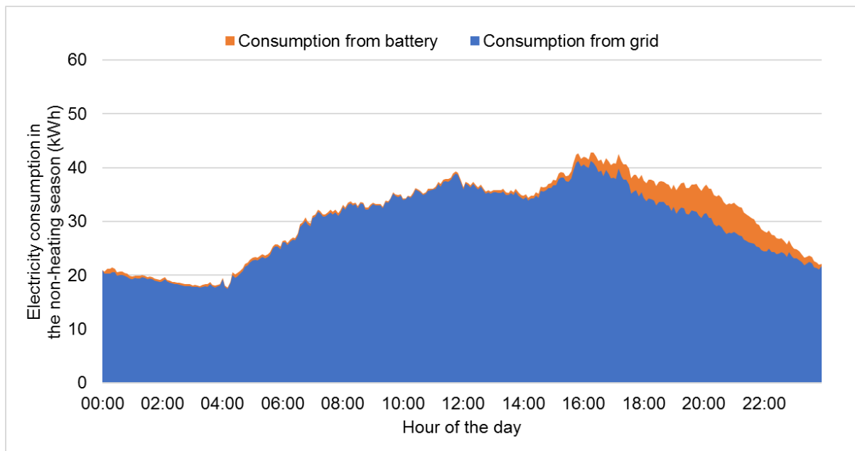
Figure 15 Electricity consumption profile in the non-heating season showing grid electricity and discharged electricity from the batteries (peak demand is between 16:00 and 18:00)
