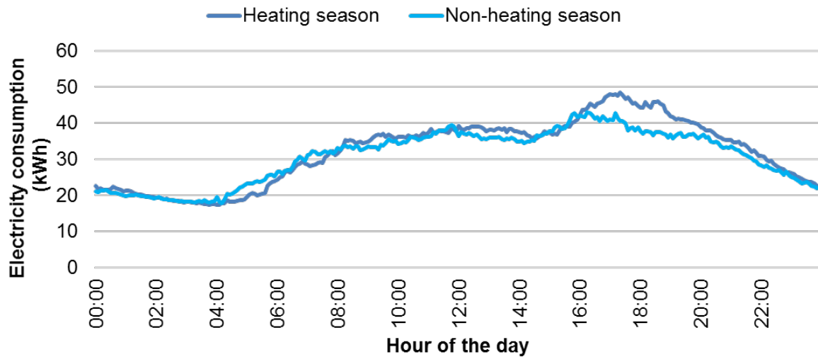
Figure 13 Electricity consumption profiles in the heating and non-heating seasons at a community level (n=74 dwellings)
