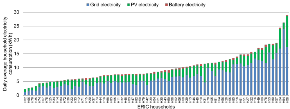
Figure 9 Daily average household electricity consumption from the grid, PV and batteries
