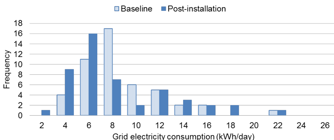
Figure 8 Histogram of grid electricity consumption estimated in the baseline period (n=4854) and measured in after the installation of the batteries (n=4874)
