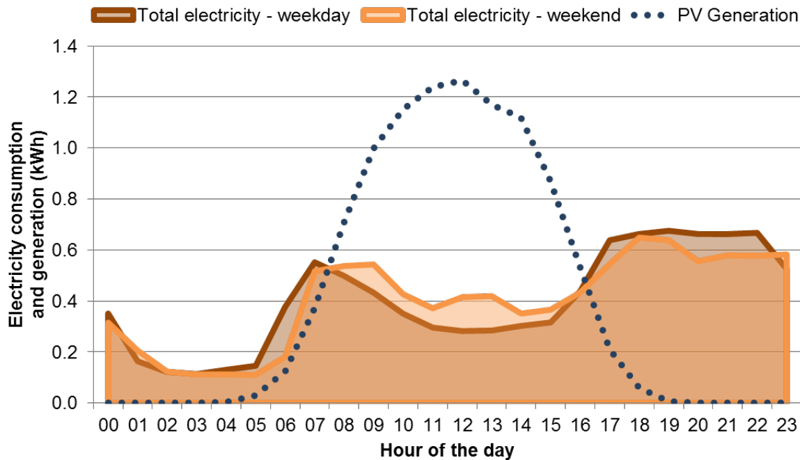
Figure 1 Electricity consumption and PV generation profiles in a UK household: household occupied in the evenings and weekends only by one family with dependent children with a daily average electricity consumption of 9 kWh (4)
