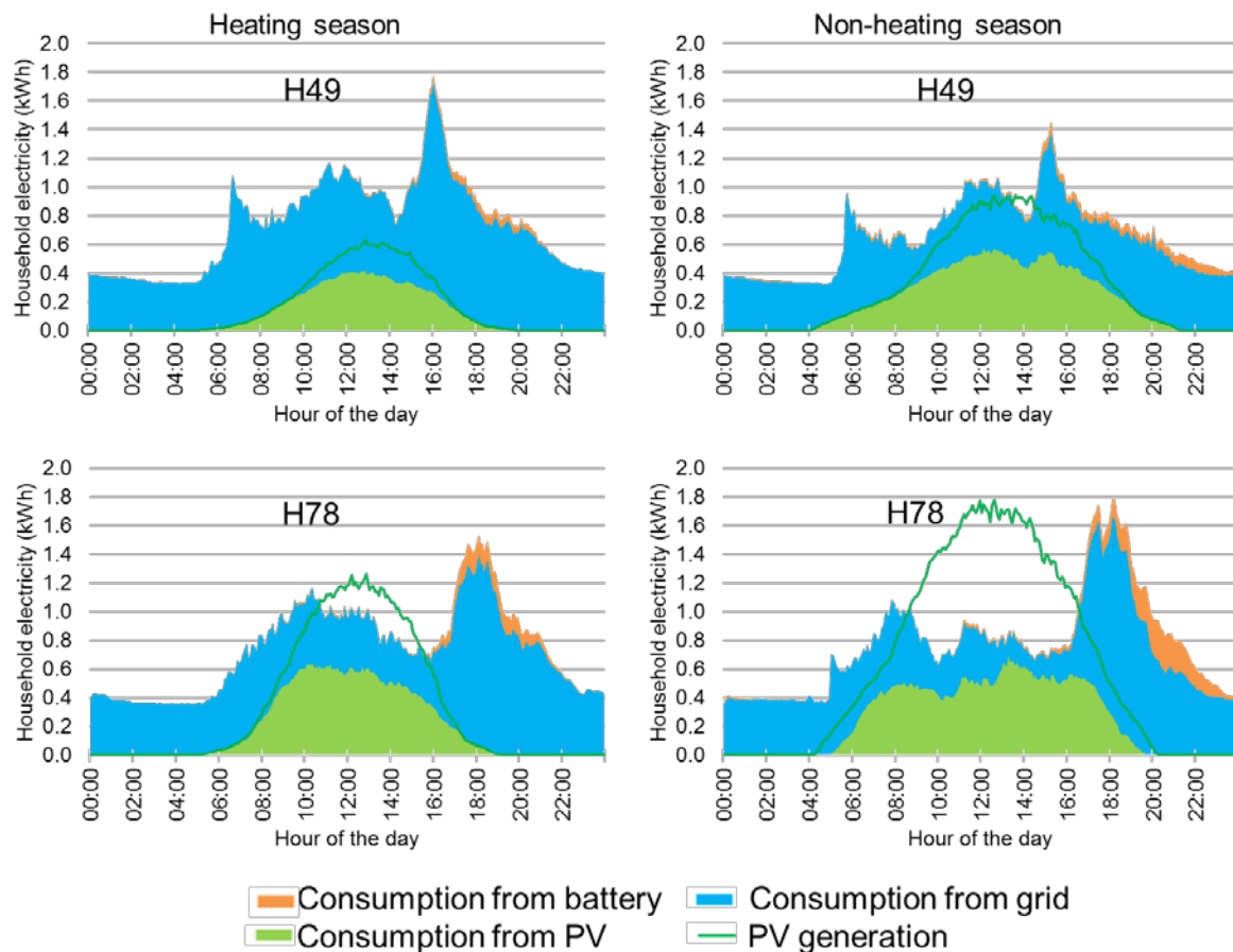
Figure 12 Household electricity consumption and generation profiles: electricity from the grid, instant consumption of PV generated electricity and PV electricity discharged from the battery in the heating season (left) and non-heating season (right) in two high consuming households
