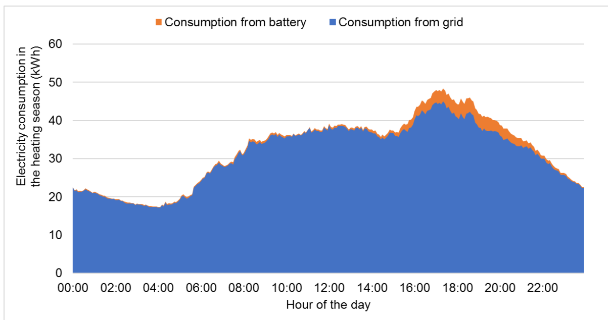
Figure 14 Electricity consumption profile in the heating season showing grid electricity and discharged electricity from the batteries (peak demand is between 17:00 and 19:00)
