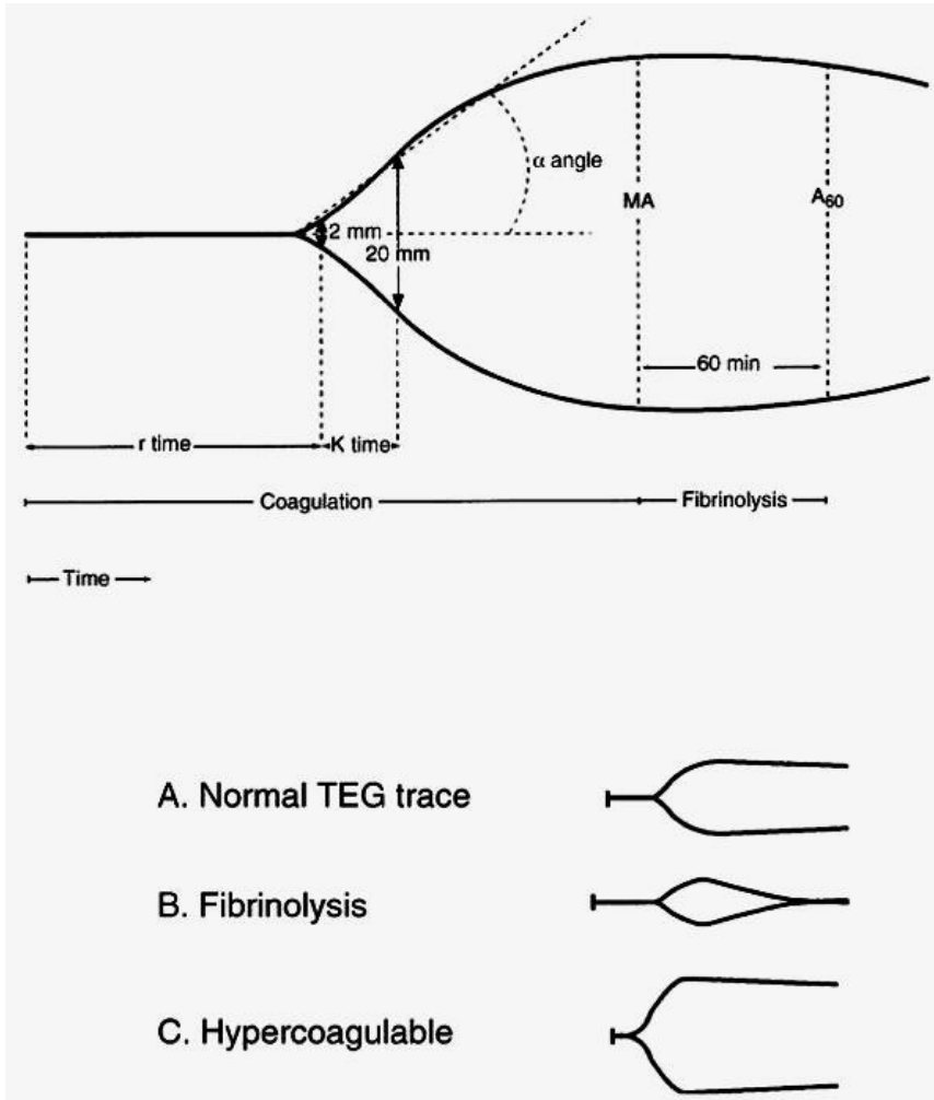
Figure 1.4.2 Thromboelastography Trace
