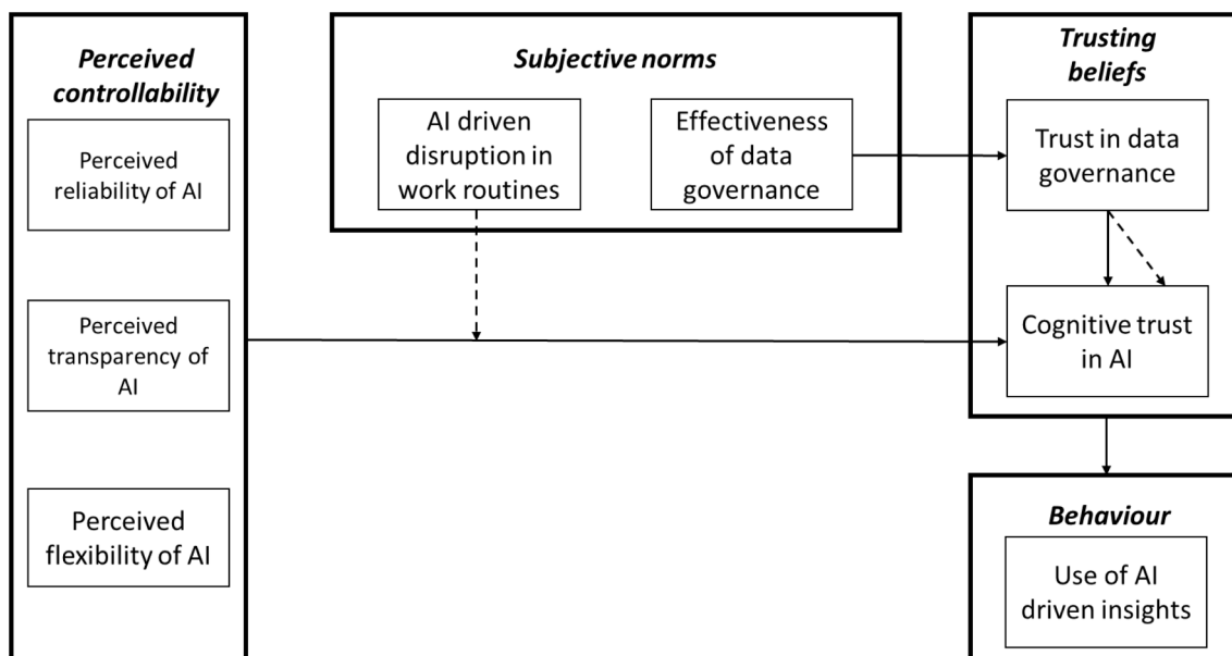
Fig. 1. Proposed framework.
