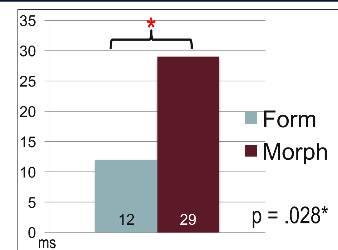
Figure 4: Comparison of degree of priming in the L2 data
