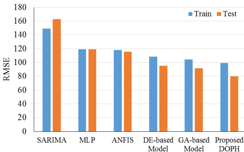
Figure 7. RMSE values for study by Chahkoutahi and Khashei (2017). Reproduced from [38], Elsevier 2017.
