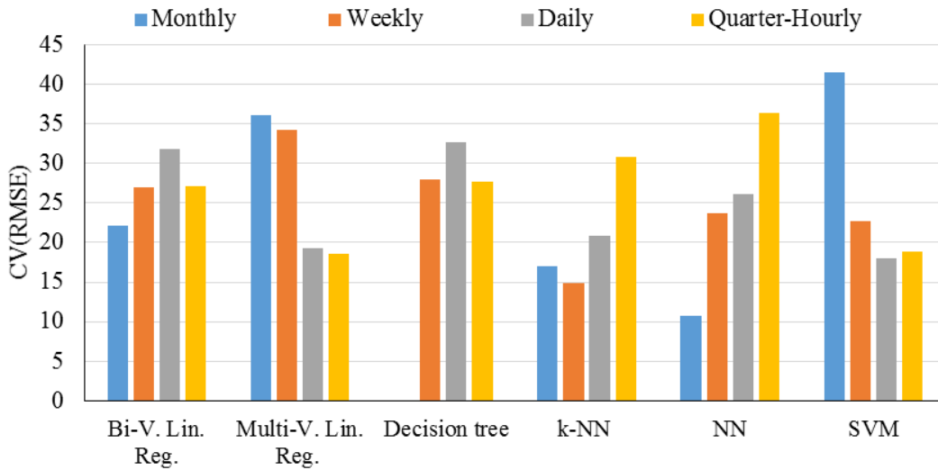
Figure 5. RMSE values for study by Callaghan et al. (2018). Reproduced from [33], Elsevier, 2018.
