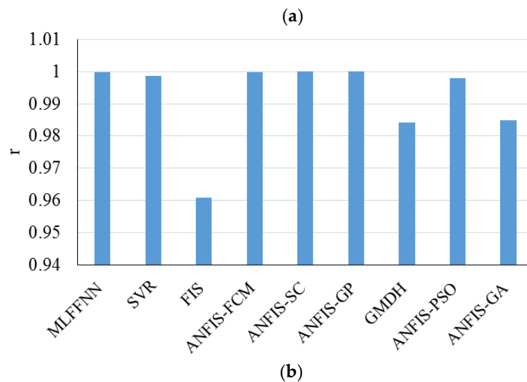
Figure 32. (a) RMSE and (b) r values for study by Khesravi et al. (2018). Reproduced from [99], Elsevier: 2018.
