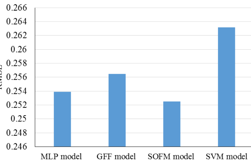
Figure 8. RMSE values for study by Kazem and Yousif (2013). Reproduced from [39], Elsevier: 2013.
