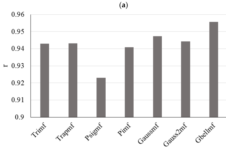
Figure 16. (a) RMSE and (b) correlation coefficient values for study by Bassam et al. (2017) reproduced from [59], Elsevier: 2017.
