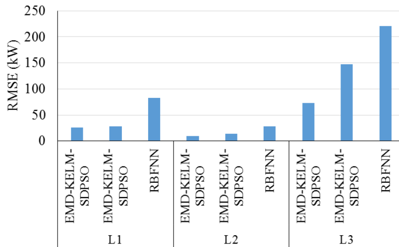
Figure 22. RMSE values for study by Deng et al. (2018). Reproduced from [80], Elsevier, 2018.
