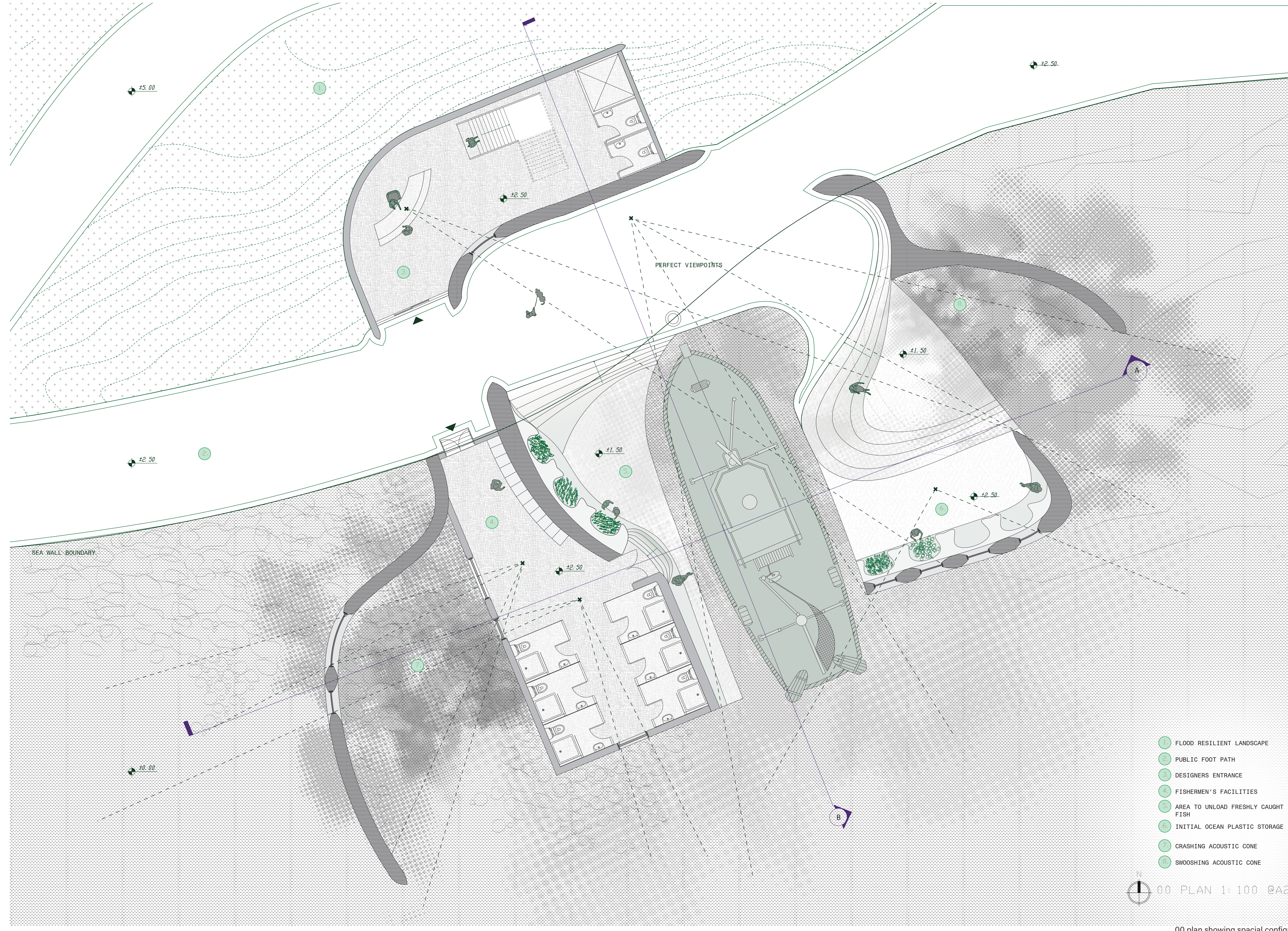
00 PLAN 1:100 @A2
