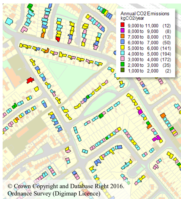
Figure 6: Baseline map – annual CO 2e emissions
