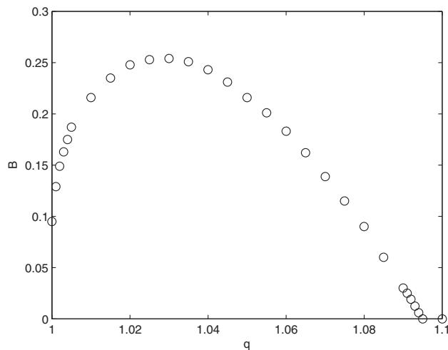
FIG. 4.9. Plot of B vs. q for m = 3 .
