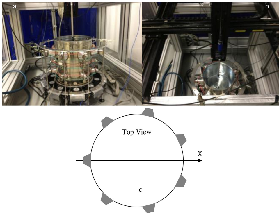
Fig. 5. Experiments of cavimeter probe spatial sensitivity: (a) the reference multifrequency cavitation vessel at NPL, (b) the cavimeter probe submerged along the centre axis of the vessel, and (c) the orientation of the cavimeter hydrophone scans.
