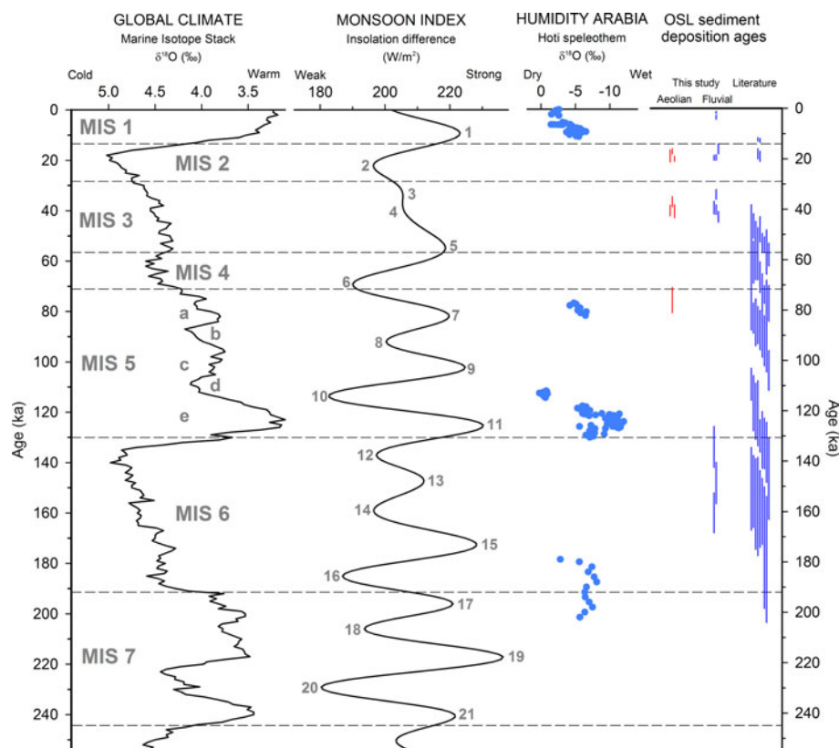
Figure 9. Summary figure displaying fluvial sediment OSL deposition ages determined within the present study and those reported in the literature (Krbetschek et al. , 2008; Parker and Rose, 2008; Atkinson et al. , 2012, 2013; Farrant et al. , 2012, 2015; Parton et al. , 2013, 2015b; Hoffmann et al. , 2015) for SE Arabia. Additionally, ages for aeolian deposits determined in the present study are displayed. The Marine Isotope Stack of Lisiecki and Raymo (2005) is shown as a measure of global climate conditions. The Monsoon Index (Leuschner and Sirocko, 2003) is given as an expression of potential theoretical climate forcing.
