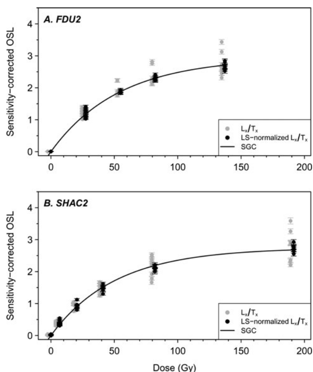
Figure 6. Two representative examples of regenerative dose points of the full SAR measurements before and after LS-normalization. The latter is used to derive the SGCs.
